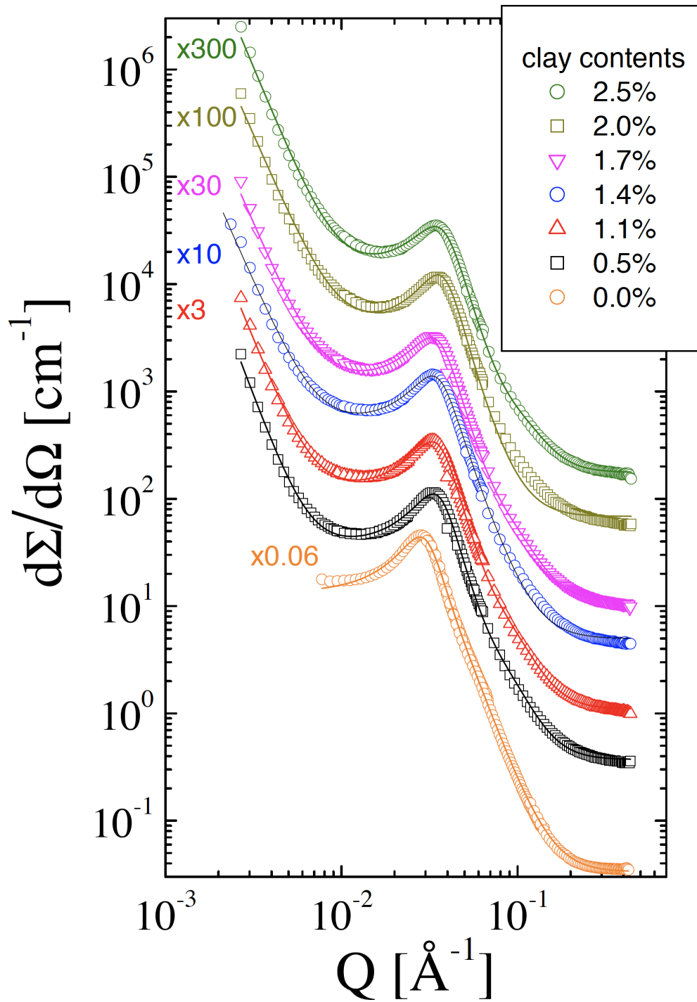
Figure D 3 The small angle scattering of microemulsions with dispersed MMT particles. For clarity, the different clay contents are shown with shifted curves according to the numbers given in the left upper corner. Most error bars are similar to the symbol size.
