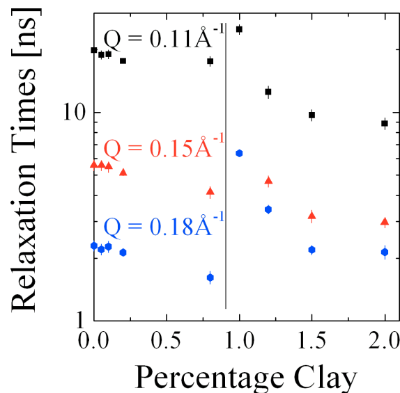
Figure 5 The relaxation times of the MMT system under film contrast with varying clay contents. A clear phase boundary is obtained at 0.9% vol clay.
