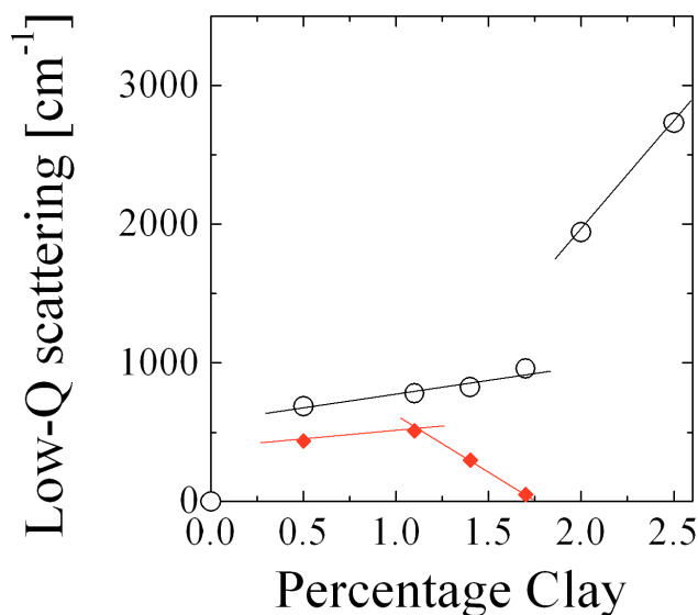
Figure G The Porod scattering at s = 0.0033 \text{ r}^{-1} as a function of the clay content. The open dots correspond to MMT dispersions, and the diamonds to LRD dispersions. The lines are guides for the eye. Most error bars are similar to the symbol size.
