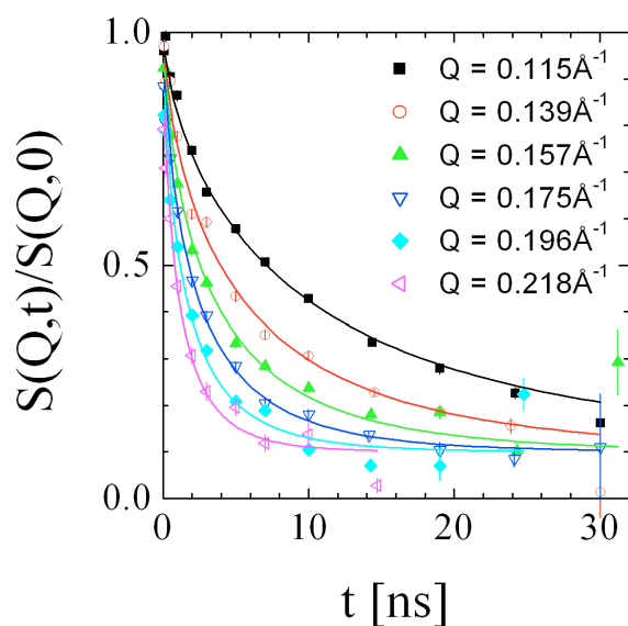
Figure H Relaxation curves of the MMT system at 1.5%vol clay with a film contrast microemulsion. The lines result from a fit of a stretched exponential with an elastic contribution of 0.1 for all s -values.
