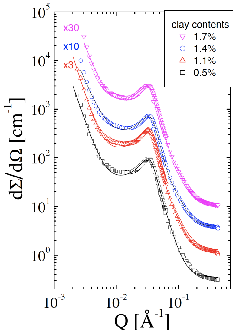
Figure 1. Small angle scattering of microemulsions with dispersed LRD particles. For clarity, the different clay contents are shown with shifted curves according to the numbers given in the left upper corner. Most error bars are similar to the symbol size.
