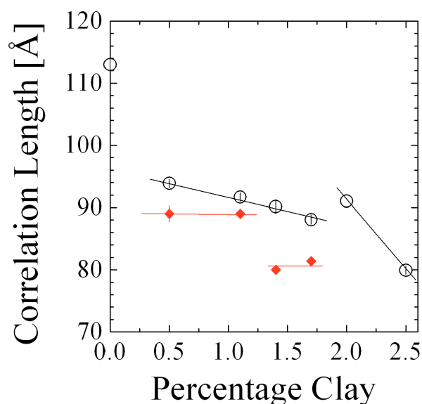
Figure 5E The correlation length of the SANS data as a function of the clay concentration. The open dots correspond to MMT dispersions, and the diamonds to LRD dispersions. The lines are guides for the eye. Most error bars are similar to the symbol size.
