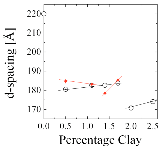
Figure 5F The d-spacing of the SANS data as a function of the clay content. The open dots correspond to MMT dispersions, and the diamonds to LRD dispersions. The lines are guides for the eye. Most error bars are similar to the symbol size.
